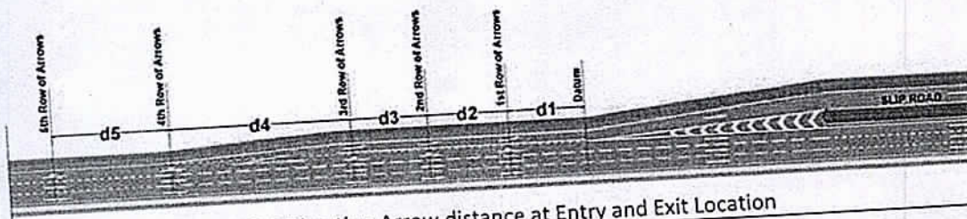
Fig 5.5 Direction Arrows
