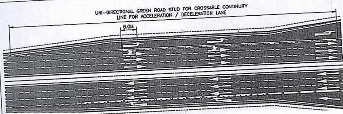
Fig 5.4 Road Stud at Merging/Diverging location
