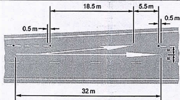
Fig 5.7 Bifurcation Arrows
