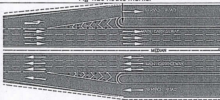
Fig 5.1 Chevron Marking
